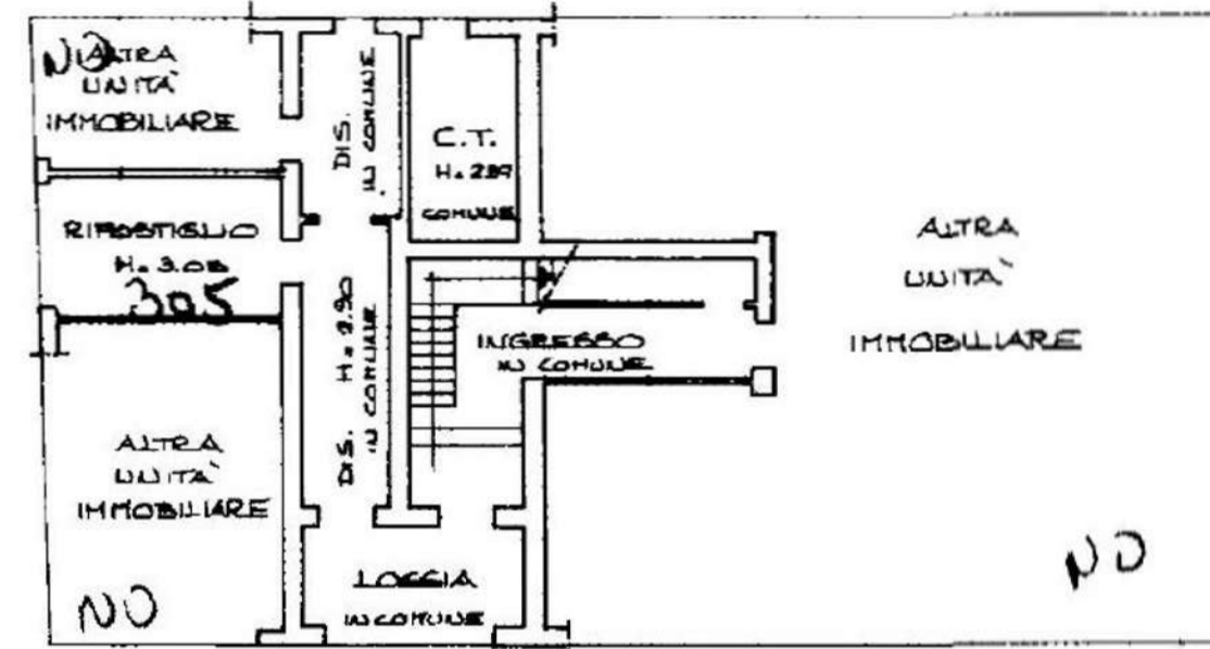
PIANO TERRA
